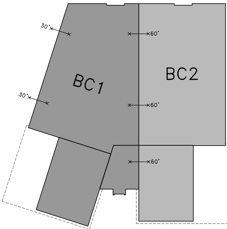
Brandcompartimering BC1 = 825 m2 BVO BC2 = 825 m2 BVO
